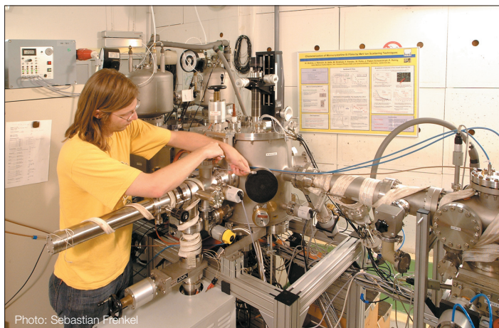
Fig. 1: The time-of-flight ERDA set up
