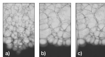
Fig. 4: X-ray radioscopes images of the evolution of argon-blown foam produced by gas injection. a) just after foam formation, b) at the end of isothermal holding (5 min), c) after solidification. Sample widths are 40 mm at the bottom.
