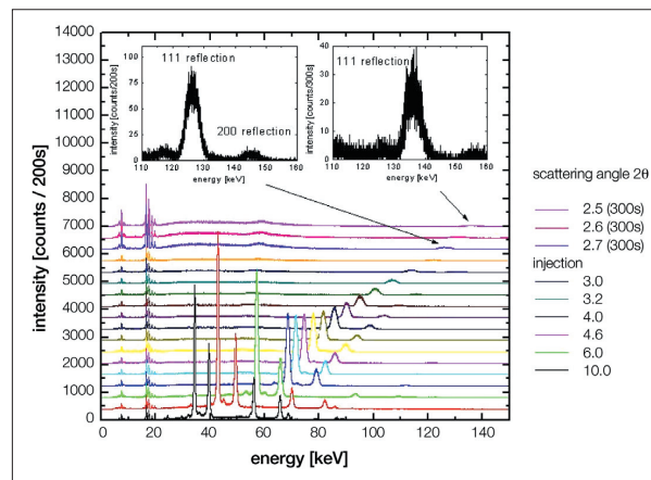
Fig. 2: Energy diffraction spectra of the alloy In 718 obtained at the materials science beamline EDDI. The measurements were performed for different scattering angles 2\theta at a wiggler field of 6 T. In this case, the peak position can be determined reliably for energies up to approximately 135 keV. With the full wiggler field of 7 T, energies of up to 150 keV can be used.
