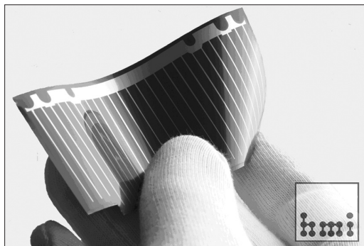
Fig. 1: Prototype of a lightweight flexible solar cell based on \text{Cu(In,Ga)Se}_2 . The total area (excluding busbar) is 27.1 \text{ cm}^2 . This type of device has reached an efficiency of 15.0% under one-sun reference illumination (AM1.5).
