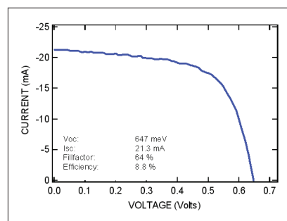
Fig. 3: AM1.5 illuminated current voltage characteristic for a ZnO/CdS/CuInS 2 /Mo solar cell prepared by reactive sputtering, T_s = 500^\circ\text{C} , r \sim 1.1 .
