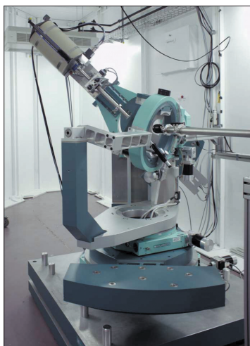
Fig. 3: MAGS, the new instrument for resonant magnetic scattering operated by the Hahn-Meitner-Institut at BESSY
