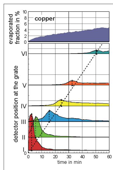
Fig. 3: Results of a copper evaporation experiment
