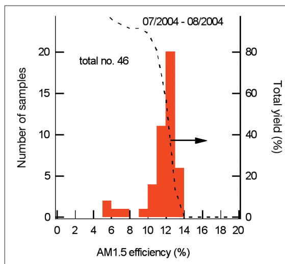
Fig. 2: Distribution of AM1.5 efficiencies of all processed 27.1 cm 2 devices of the Hahn-Meitner-Institut baseline over a period of two month. The narrow distribution reflects the high level of process reproducibility of the baseline process for flexible solar cells. The dashed line depicts the number of samples above a respective efficiency threshold value.
