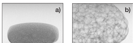
Fig. 3: X-ray radioscopes images of a) Al99.7+0.5 wt% TiH 2 foamed under 8 bar in air, b) additional expansion of a) after release from 8 bar to 1 bar with -0.2 \text{ bar/s}
