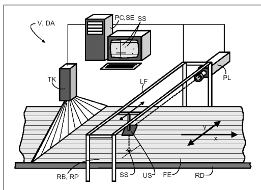
Fig. 2: Sketch of a suggested in-line machine for automatic module diagnosis and repair using a Thermocamera (TK) and a laser (PL). The substrate is moving in direction of x. Due to their higher power dissipation, local shunts (SS) are detected by the thermocamera and recorded by a computer (PC). In case of a local shunt detection, the mirror (US) is positioned above the shunt and a laser puls is directed onto the module surface at the defected area. The transparent conductive ZnO layer is selectively removed.
