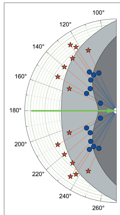
Fig. 3: Angular distribution of Auger-intensity ratios (in polar coordinates) for L^2VV to L^1VV (red asterisks) as well as for L^3VV to L^1VV (blue circles) line intensities from atomically clean Al surfaces. The green arrow indicates the incident direction of the 592 MeV Au^{48+} projectile ions.
