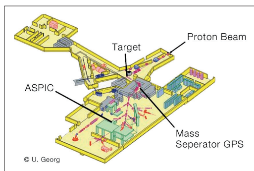
Fig. 2: The on-line mass separator ISOLDE at CERN. The ultra-high vacuum (UHV) chamber ASPIC (Apparatus for Surface Physics and Interfaces at CERN) is located in the center of the experimental hall. It is connected to the mass separator by a UHV beam line. (Courtesy of U. Georg, ISOLDE)
