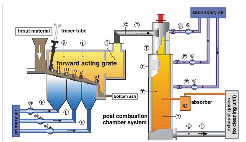
Fig. 1: Technical flowchart of the forward-acting grate plant (● radiation detector)
