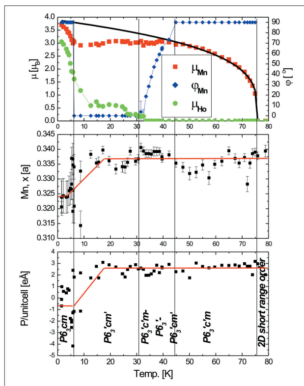
Fig. 3: Intra planar antiferromagnetic \text{Ho} ordering contradicts the symmetry P6_3c'm' , a new symmetry P6_3cm is formed. The different coupling between the planes, \delta_3 -axis instead of \delta_3' -axis, requires different magnetic exchange paths, this leads to a change in the electric polarization: The O-Mn-O axis of the coordination polyhedra is shifted.
