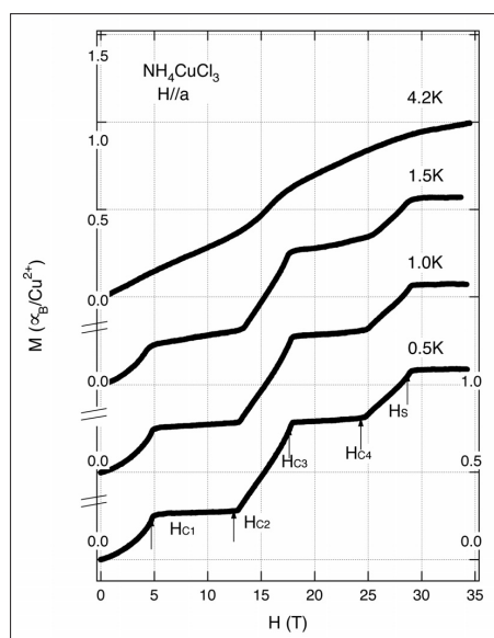
Fig. 1: Magnetisation curves of \text{NH}_4\text{CuCl}_3 measured at different temperatures with H \parallel a , from Ref. [5]
