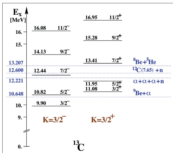
Fig. 2: Energy levels of ^{13}\text{C} grouped into rotational bands (parity doublets), the K -quantum numbers is indicated. The threshold energies for structure components related to the asymptotic cluster-structure of states are shown (from ref. [5]).
