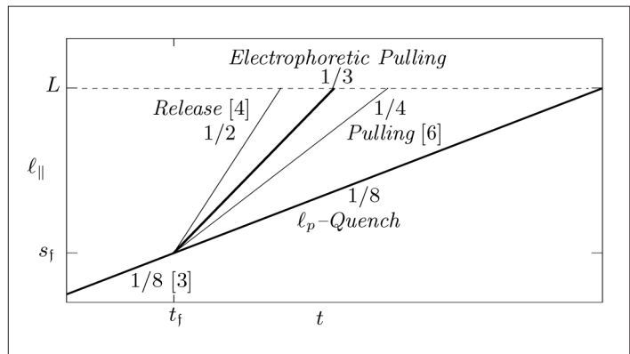
Fig. 3: Double-logarithmic sketch of the tension propagation laws l_{||}(t) \propto t^z . At a force dependent time t_f they cross over from a universal short-time regime to (problem-specific) tension-dominated intermediate regimes. The propagation ends when the tension has spread over the whole filament, l_{||}(t) \approx L .
