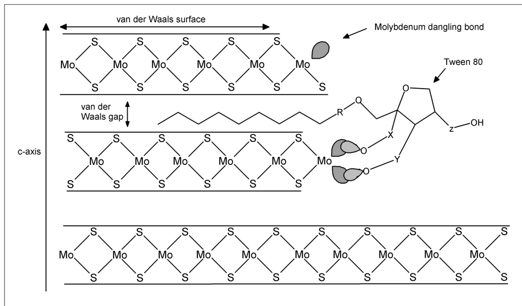
Fig. 1: Schematic figure of the different crystal surfaces in MoS 2 and possible adsorption mechanism of Tween 80 and related compounds (X, Y and Z are side chains of the -(O-CH_2-CH_2)- -type with different lengths).
