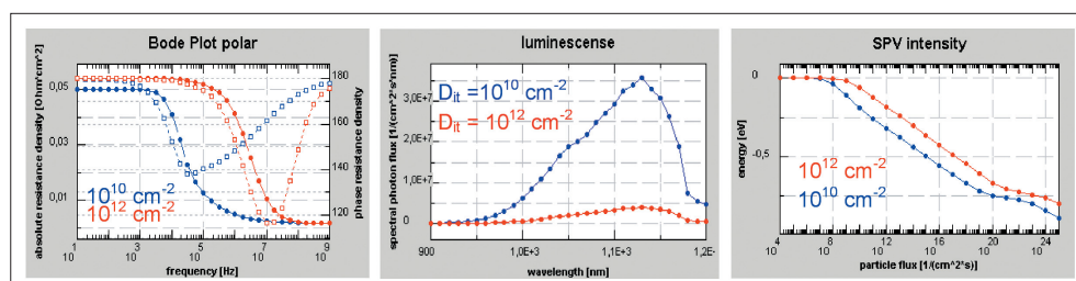
Fig. 3: Screenshots of typical AFORS-HET Output: Open-circuit Impedance (left), Photoluminescence (middle) and illumination intensity dependend Surface Photovoltage (right), simulated for a-Si(n)/c-Si(p) solar cell structures, assuming two different a-Si/c-Si interface state densities D_{it} = 10^{10} \text{ cm}^{-2} and 10^{12} \text{ cm}^{-2} .
