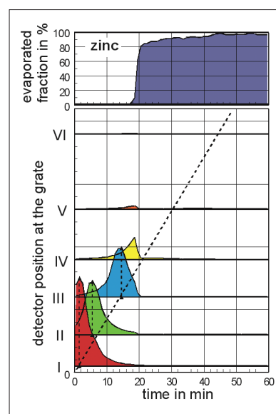
Fig. 4: Results of a zinc evaporation experiment
