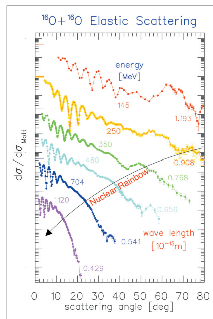
Fig. 3: Data of elastic scattering of ^{16}\text{O} + ^{16}\text{O} at different incident energies as indicated at the data. The effect of nuclear rainbow scattering is observed at large scattering angles.
