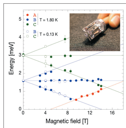
Fig.3: Field dependence of the spin dynamics in \text{NH}_4\text{CuCl}_3 measured at Q=(0\ 0\ 1) , T=1.8 K and T=0.13 K. Inset: Six coaligned \text{NH}_4\text{CuCl}_3 single crystals on an Al sample holder. The individual crystals are wrapped into Al foil and glued at the top and bottom onto adjustable Al plates. The arrangement fits into Hahn-Meitner-Institut's 15-T cryomagnet for neutron scattering experiments.
