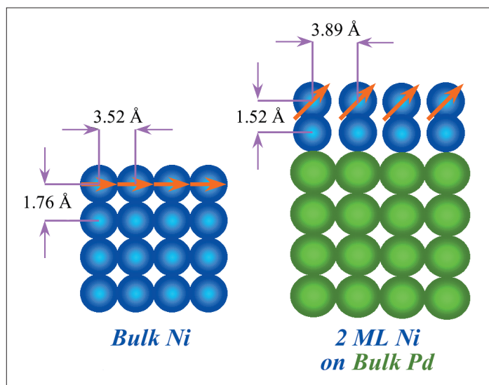
Fig. 3: Lattice parameters are shown for a bulk Ni single crystal surface (blue), the Ni surface magnetisation is in the plane, shown by the red arrows (left). However, 2 MLs Ni grown on Pd(001) is lattice expanded in the plane and compressed in the out-of-plane direction, the magnetisation was measured to be canted out of the plane (right).
