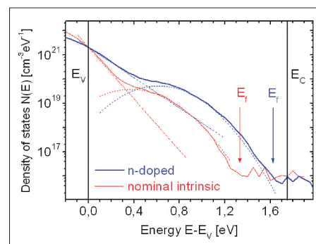
Fig. 2: Measured photoelectron yield spectroscopy data for nominal intrinsic and n-doped a-Si:H. The results are used to specify the density of states within the thin amorphous silicon layers.
